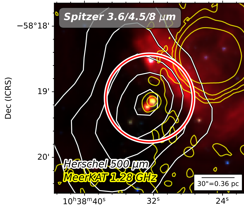
I10365-5803 (G286.208+0.171)
