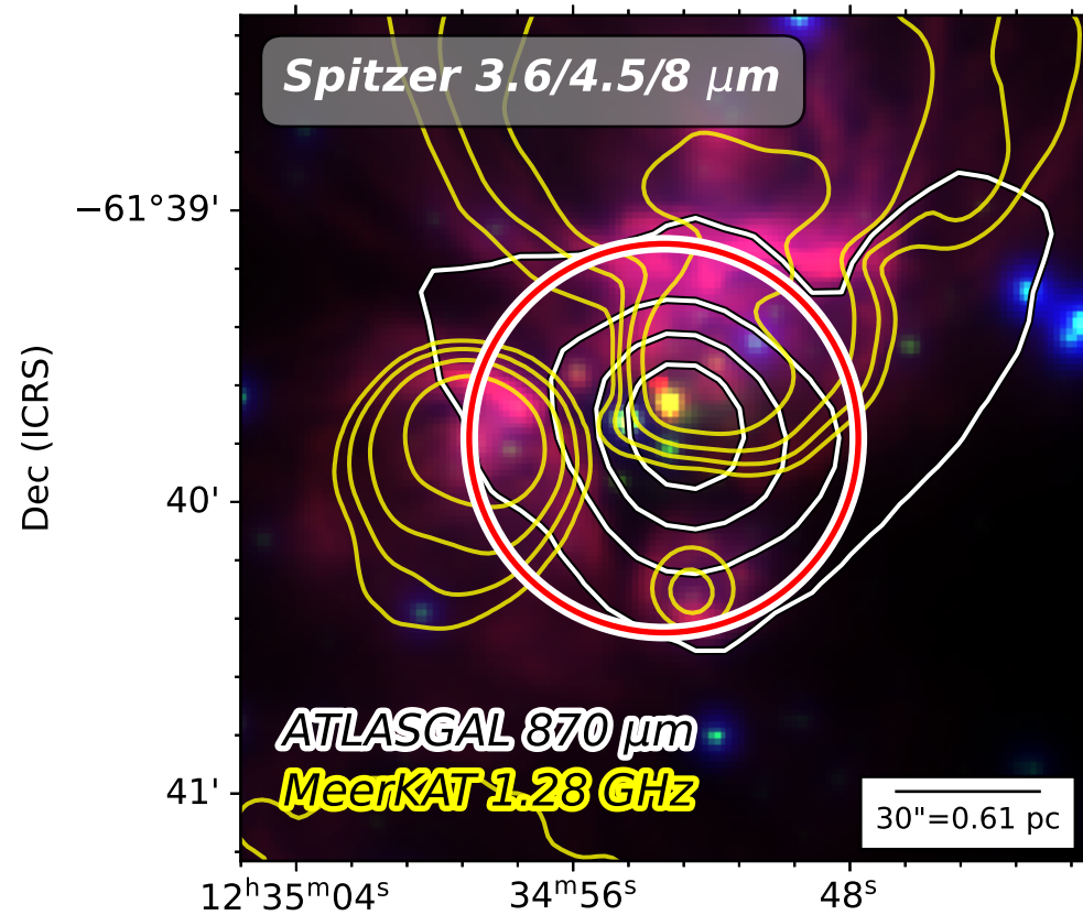
I12320-6122 (G300.969+1.146)
