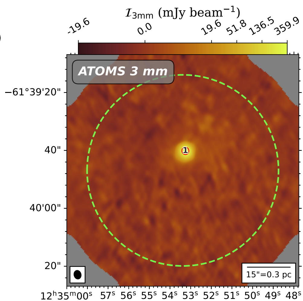
I12320-6122 (G300.969+1.146)
